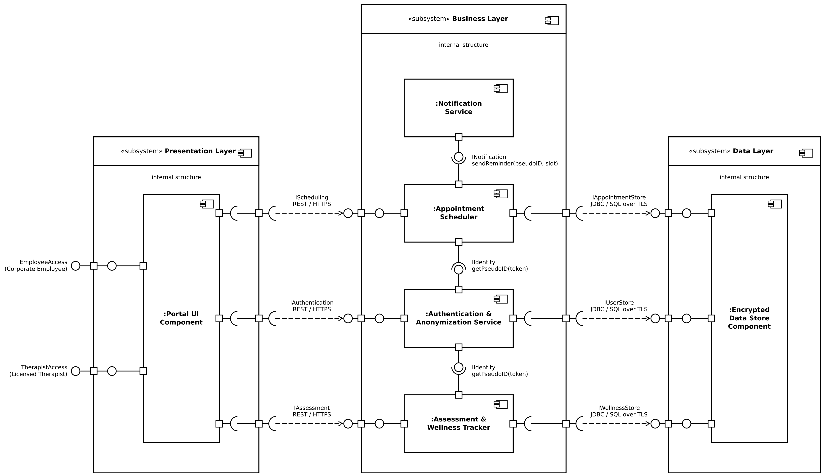
Corporate Mental Wellness & Counseling Platform UML component diagram with three layered subsystems - Presentation, Business and Data.
